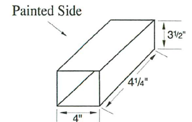
DOWNPOUT W/O KICKOUT
