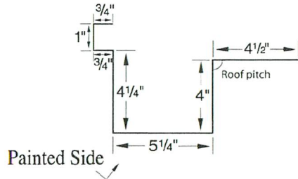
BOX EAVE GUTTER
