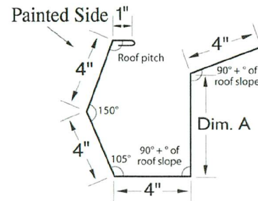
SCULPTURED GUTTER
