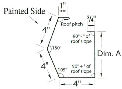
STANDARD GUTTER
