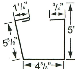
ECONOMY GUTTER
