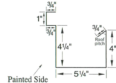
BOX HANG-ON GUTTER
