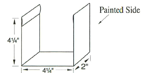
DOWNPOUT STRAP
