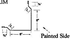
RAKE & CORNER
