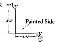
INSIDE CORNER
