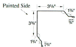
OUTSIDE CORNER
