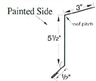
LONG EAVE TRIM
