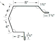
HI-SIDE EAVE TRIM
