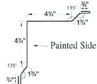
INSIDE CORNER
