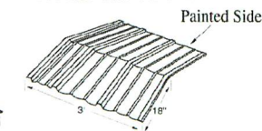
FORMED RIDGECAP
