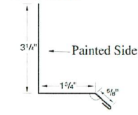
BASE TRIM
