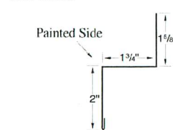
ZEE TRIM
