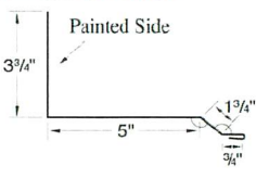
TRANSITION TRIM
