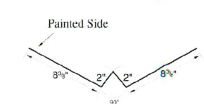
COMMERCIAL VALLEY
