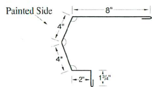
HI-SIDE EAVE TRIM
