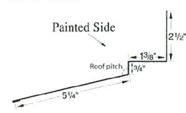
TIE IN TRIM
