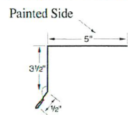
SHORT EAVE TRIM
