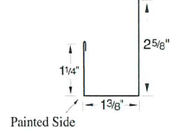
HEAD TRIM
