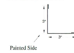
OUTSIDE ANGLE 3X3
