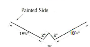
EXTENDED VALLEY
