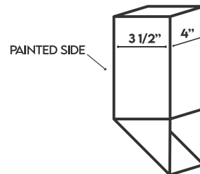
DOWNSPOUT WITH KICKOUT
