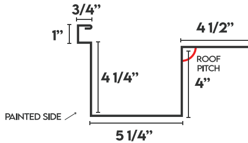
ECONOMY GUTTER
