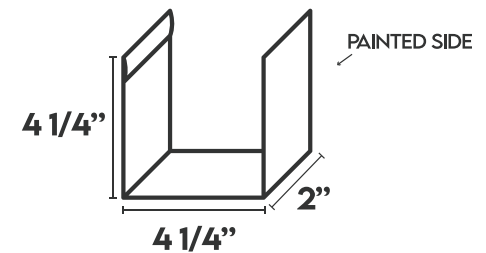
DOWNSPOUT STRAP
