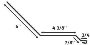
UNIVERSAL ENDWALL
