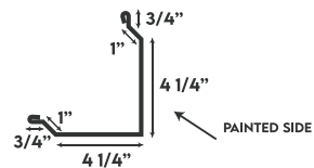
RAKE & CORNER
