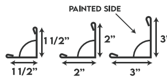
INSIDE ANGLE
