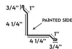
INSIDE CORNER
