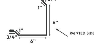
GABLE TRIM
