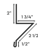
COMMERCIAL RAT GUARD
