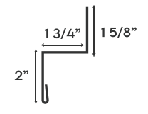
ZEE TRIM
