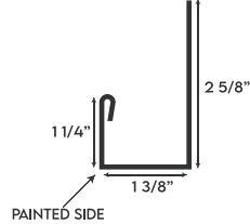
HEAD TRIM
