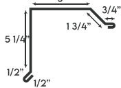
ECONOMY RAKE
