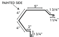
RAKE TRIM
