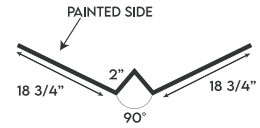
EXTENDED VALLEY
