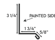
BASE TRIM
