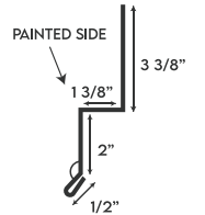
ZEE TRIM
