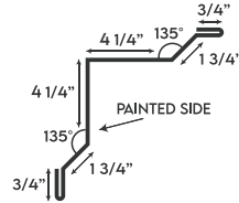
INSIDE CORNER
