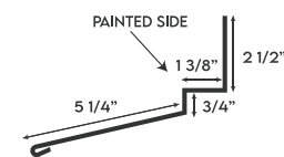
TIE IN TRIM
