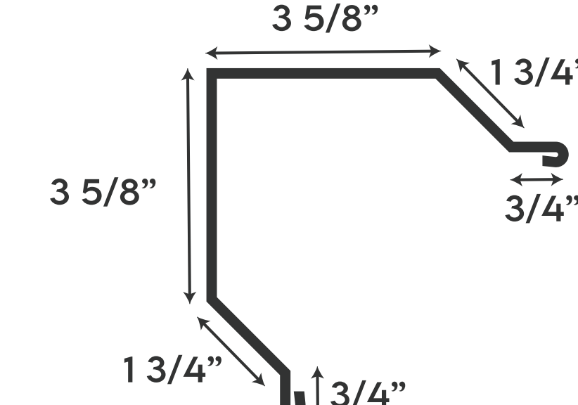
OUTSIDE CORNER
