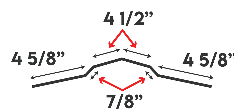
RIDGECAP
