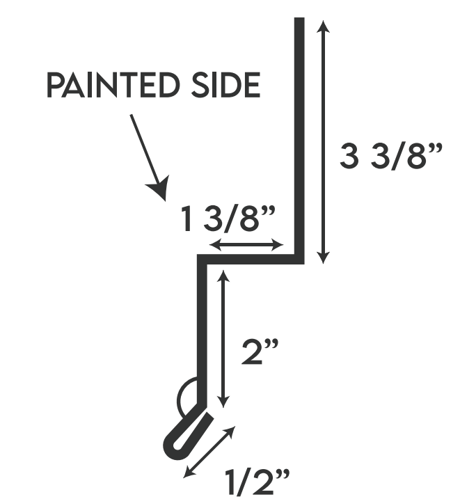
ZEE TRIM
