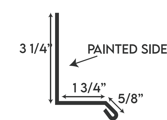
BASE TRIM
