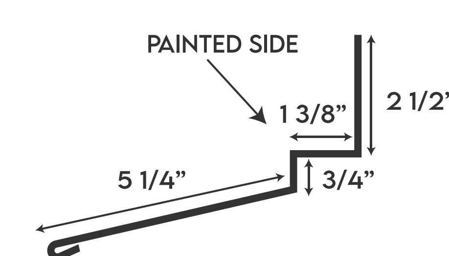
TIE IN TRIM
