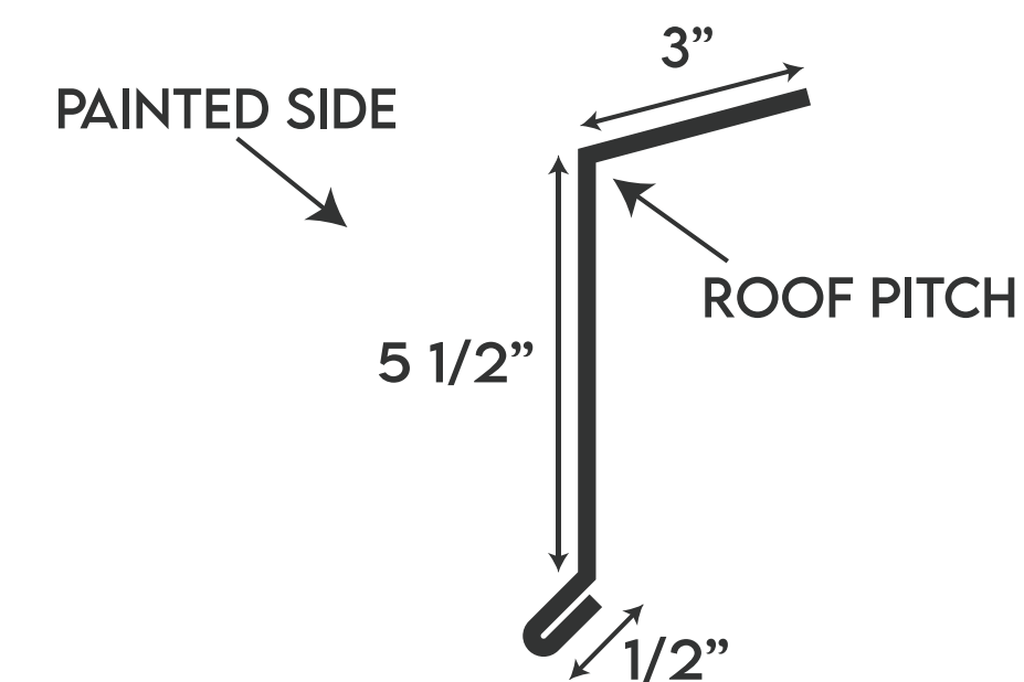
LONG EAVE TRIM
