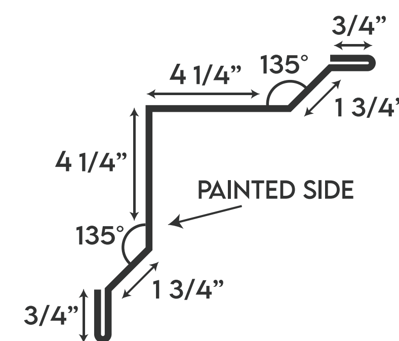
INSIDE CORNER
