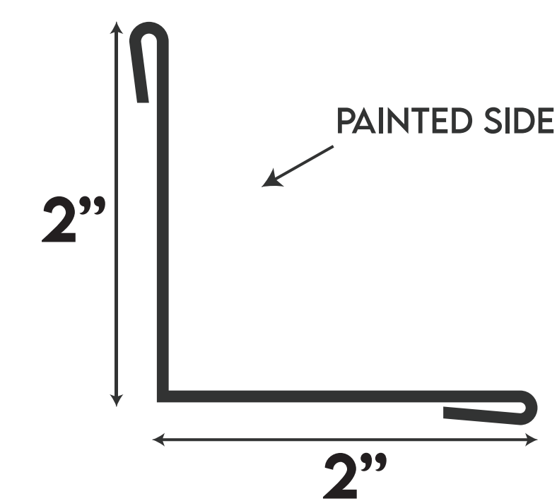
INSIDE ANGLE 2X2
