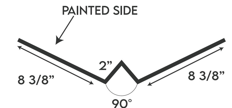
COMMERCIAL VALLEY
