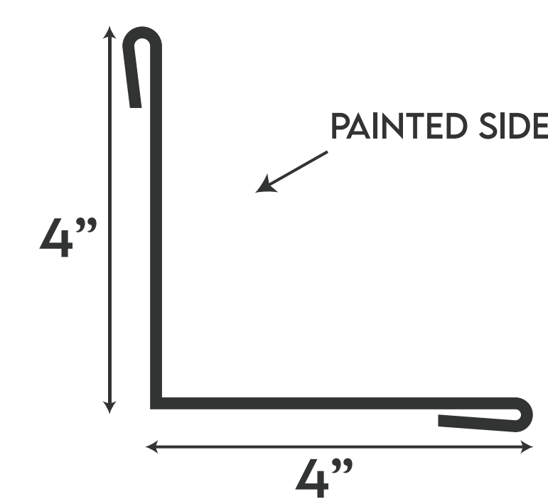
INSIDE ANGLE 4X4
