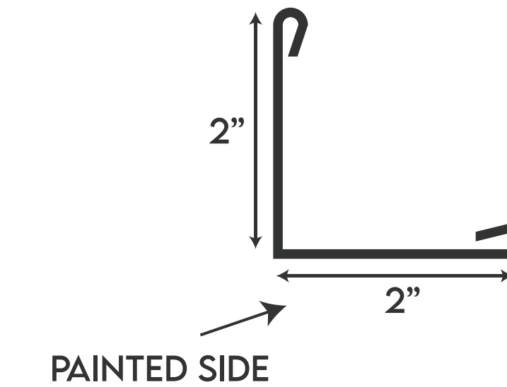
OUTSIDE ANGLE 2X2
