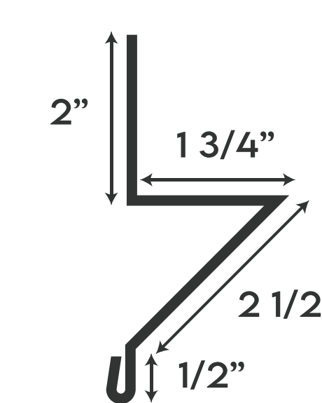
COMMERCIAL RAT GUARD
