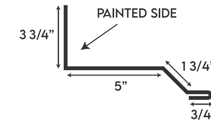
TRANSITION TRIM
