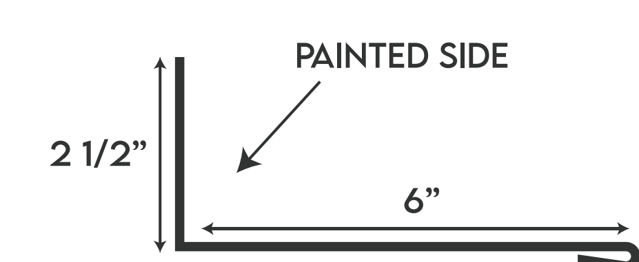
SIDEWALL TRIM
