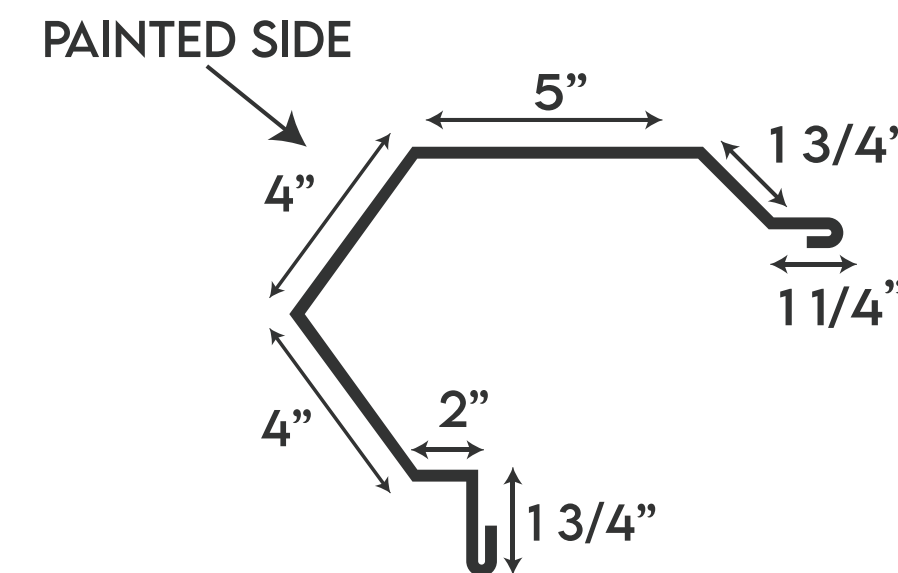
RAKE TRIM
