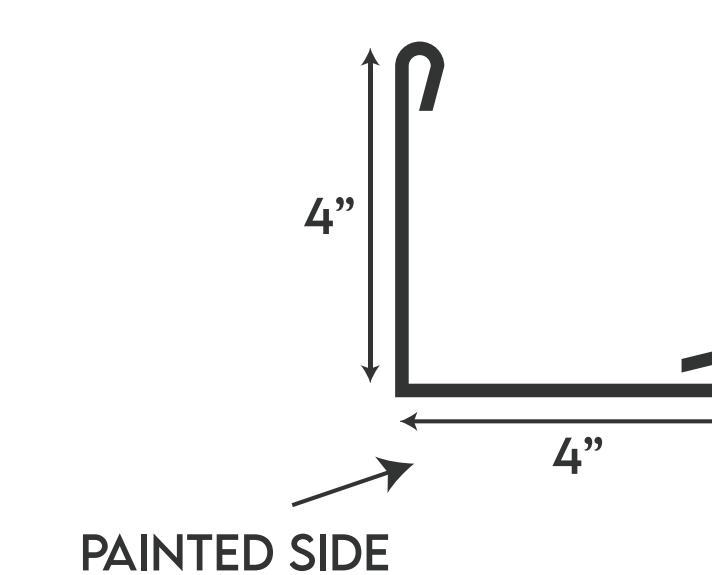
OUTSIDE ANGLE 4X4
