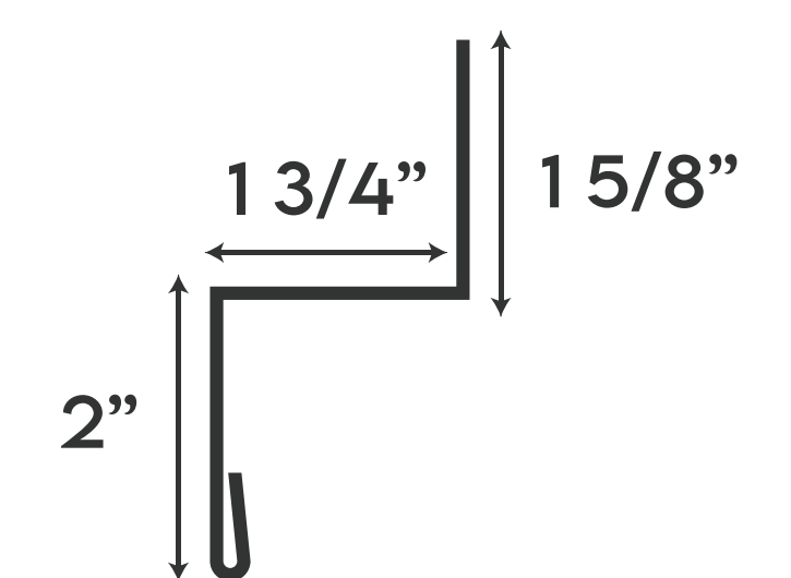
ZEE TRIM
