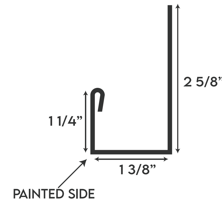
HEAD TRIM
