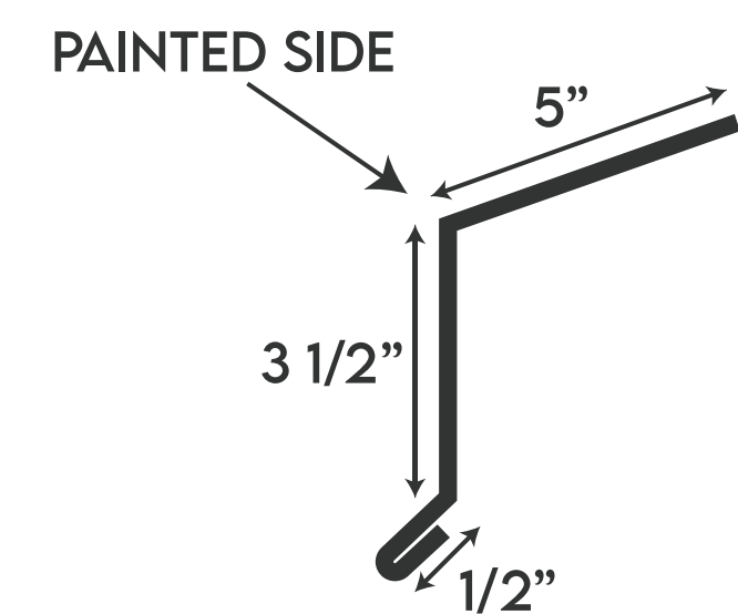
SHORT EAVE TRIM
