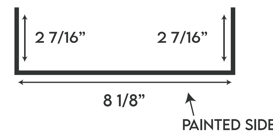
JAMB COVER/HEADER
