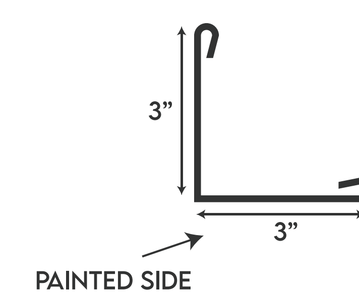
OUTSIDE ANGLE 3X3
