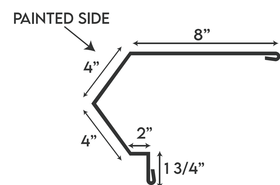
HI-SIDE EAVE TRIM
