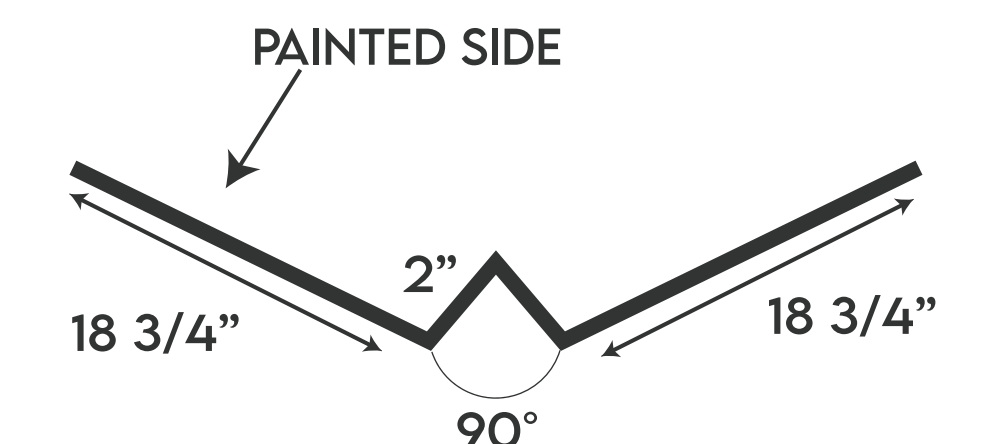
EXTENDED VALLEY
