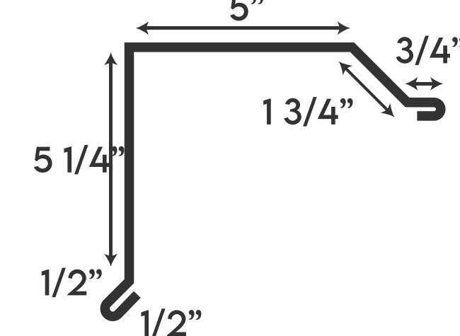
ECONOMY RAKE
