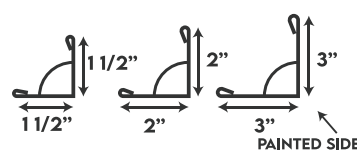
SINGLE ANGLE
