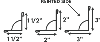
INSIDE ANGLE
