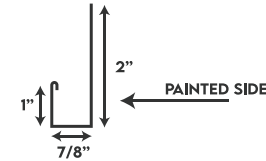
J-TRIM
