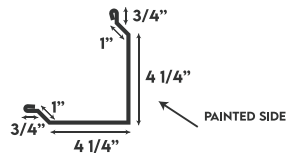
RAKE & CORNER
