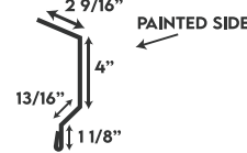
FASCIA
