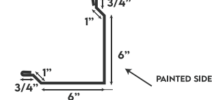
GABLE TRIM
