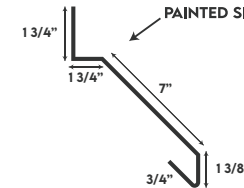
GABLE TRIM
