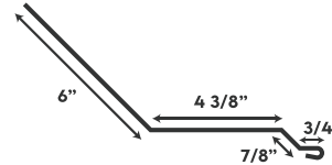
UNIVERSAL ENDWALL
