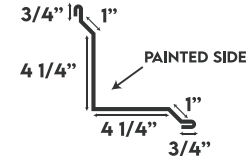
INSIDE CORNER
