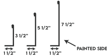
POST TRIM
