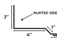
UNIVERSAL SIDEWALL
