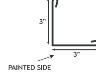
OUTSIDE ANGLE 3X3
