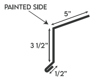
SHORT EAVE TRIM
