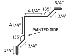
INSIDE CORNER
