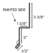
ZEE TRIM
