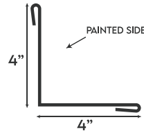
INSIDE ANGLE 4X4
