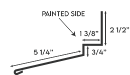
TIE IN TRIM
