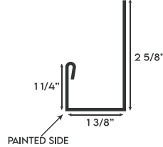
HEAD TRIM
