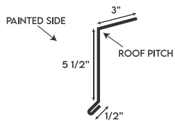
LONG EAVE TRIM
