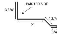
TRANSITION TRIM
