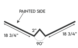
EXTENDED VALLEY
