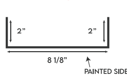
JAMB COVER/HEADER
