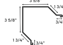
OUTSIDE CORNER
