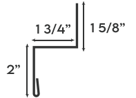
ZEE TRIM
