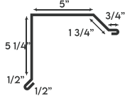
ECONOMY RAKE
